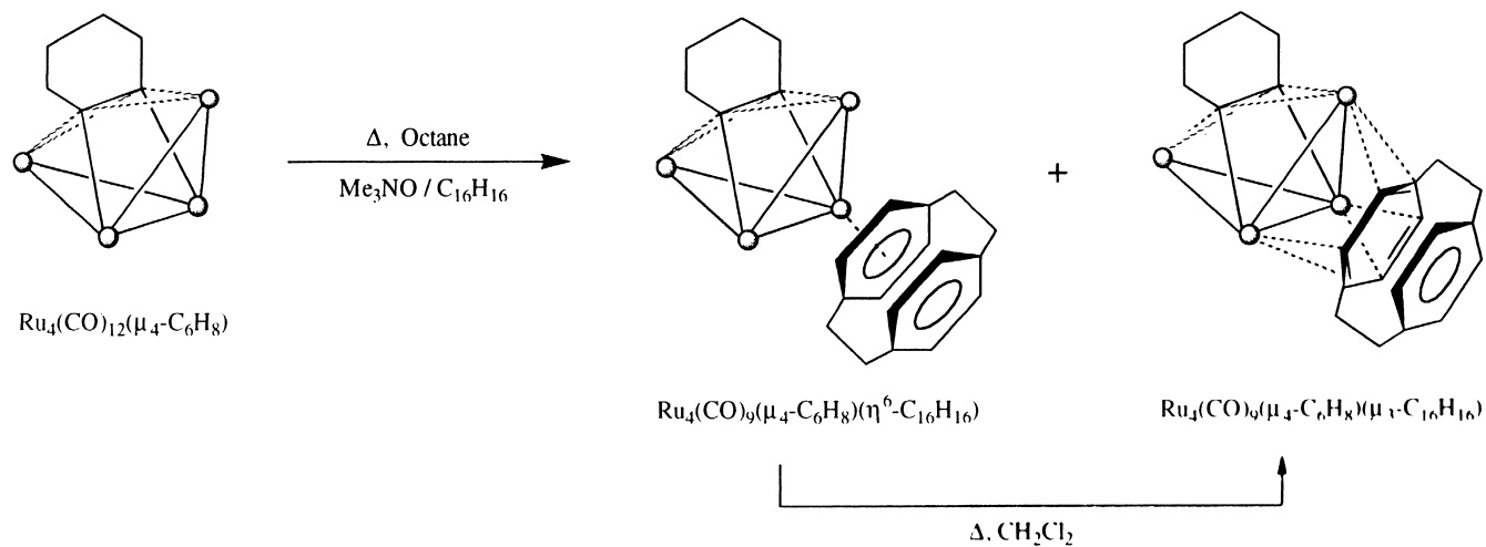
Scheme 4. Reaction of \text{Ru}_4(\text{CO})_{12}(\mu_4\text{-C}_6\text{H}_8) with [2.2]paracyclophane.
