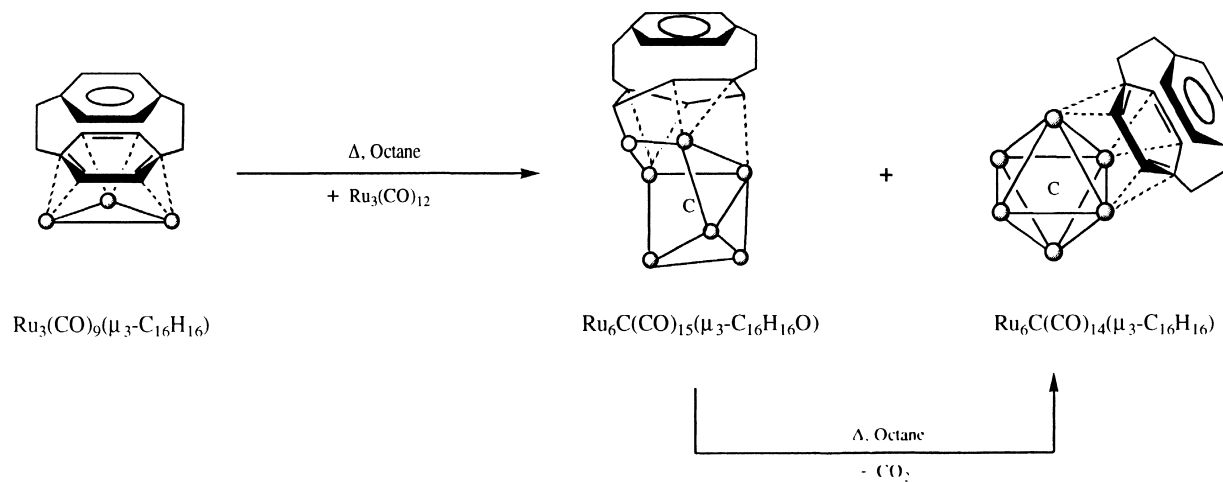
Scheme 2. The formation of \text{Ru}_6\text{C}(\text{CO})_{14}(\mu_3\text{-C}_{16}\text{H}_{16}) .
