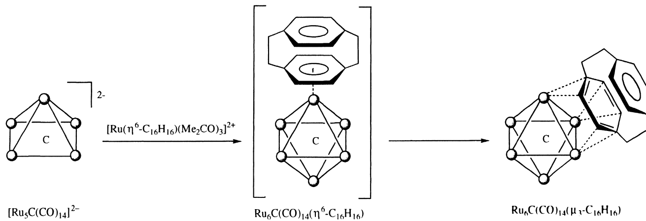
Scheme 11. Reaction of [\text{Ru}_5\text{C}(\text{CO})_{14}]^{2-} with [\text{Ru}(\eta^6\text{-C}_{16}\text{H}_{16})(\text{MeCN})_3]^{2+} .
