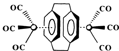
Fig. 2. \{\text{Cr}(\text{CO})_3\}_2(\eta^6\text{-}\eta^6\text{-C}_{16}\text{H}_{16}) .
