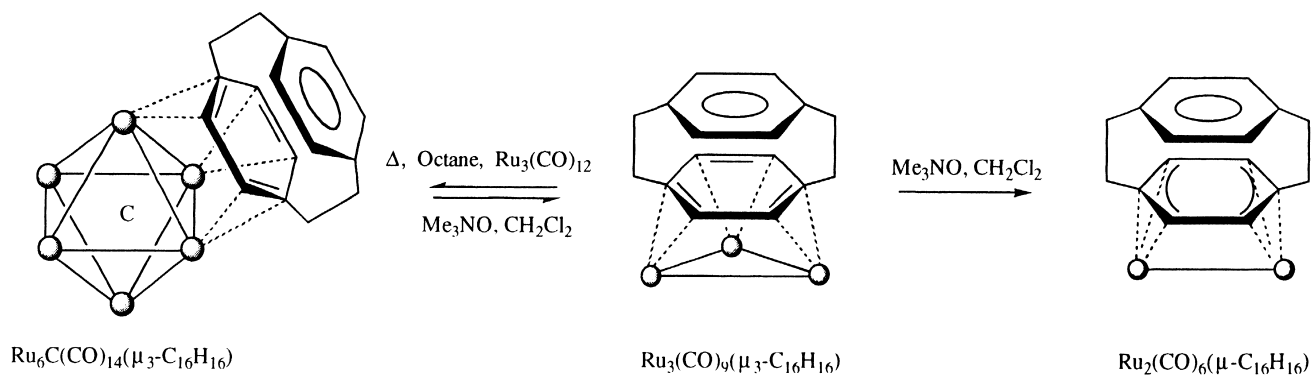
Scheme 6. Reactions involving a change in nuclearity.
