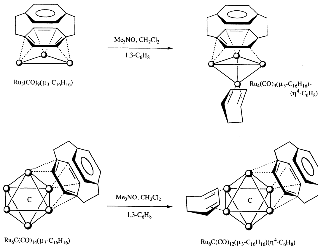
Scheme 9. Reaction of \text{Ru}_3(\text{CO})_9(\mu_3\text{-C}_{16}\text{H}_{16}) and \text{Ru}_6\text{C}(\text{CO})_{14}(\mu_3\text{-C}_{16}\text{H}_{16}) with cyclohexa-1,3-diene.
