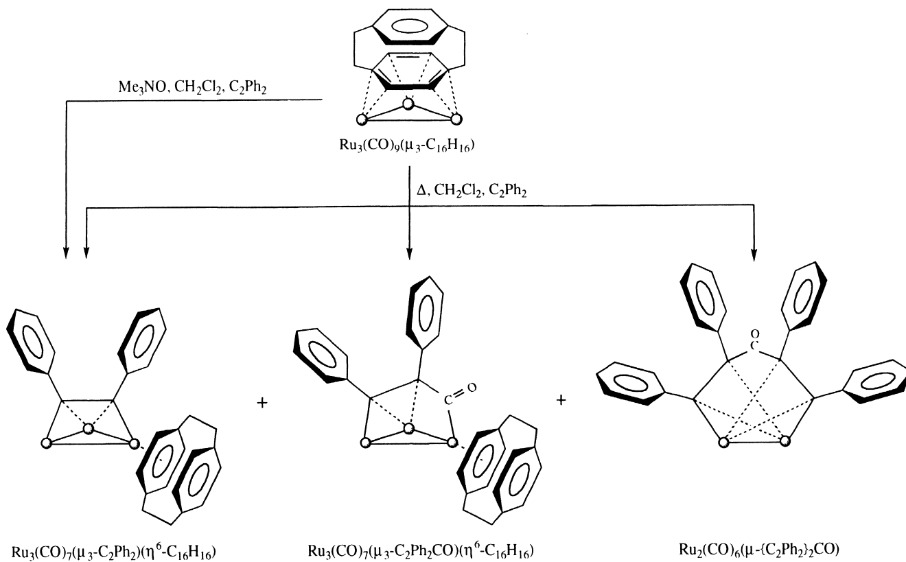
Scheme 8. Reactions of \text{Ru}_3(\text{CO})_9(\mu_3\text{-C}_{16}\text{H}_{16}) with diphenylacetylene.
