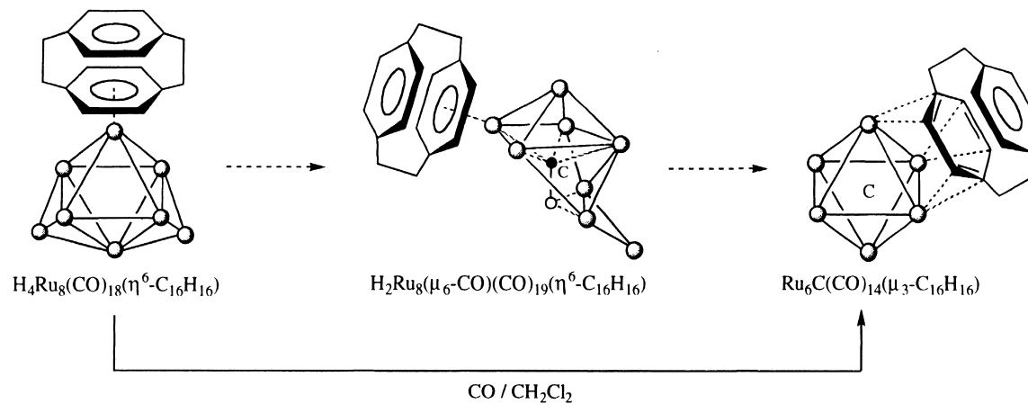
Scheme 3. The conversion of \text{Ru}_8(\mu\text{-H})_4(\text{CO})_{18}(\eta^6\text{-C}_{16}\text{H}_{16}) into \text{Ru}_6\text{C}(\text{CO})_{14}(\mu_3\text{-C}_{16}\text{H}_{16}) , showing \text{Ru}_8(\mu\text{-H})_2(\mu_6\text{-}\eta^2\text{-CO})(\text{CO})_{19}(\eta^6\text{-C}_{16}\text{H}_{16}) as a possible reaction intermediate.
