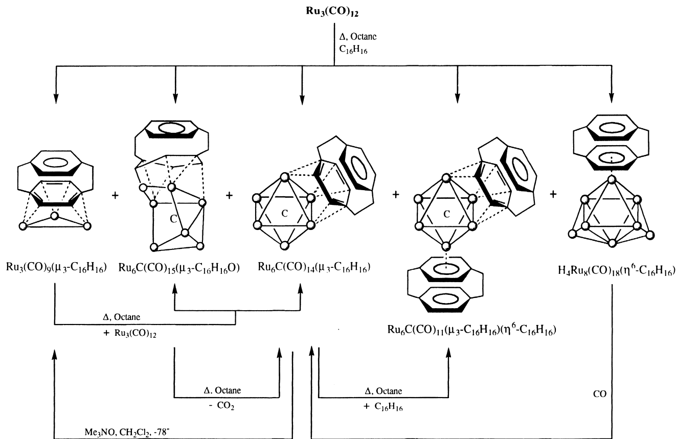
Scheme 1. The reaction of \text{Ru}_3(\text{CO})_{12} with [2.2]paracyclophane. Carbonyl ligands are omitted for clarity.
