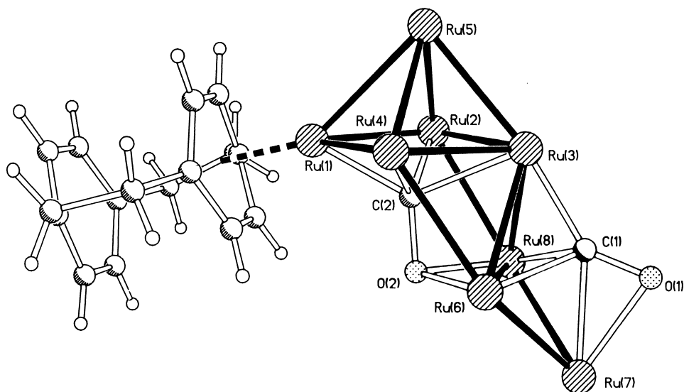
Fig. 11. The solid-state molecular structure of \text{Ru}_8(\mu_6\text{-}\eta^2\text{-CO})(\mu_4\text{-}\eta^2\text{-CO})(\text{CO})_{18}(\eta^6\text{-C}_{16}\text{H}_{16}) . The terminal COs have been omitted for clarity.
